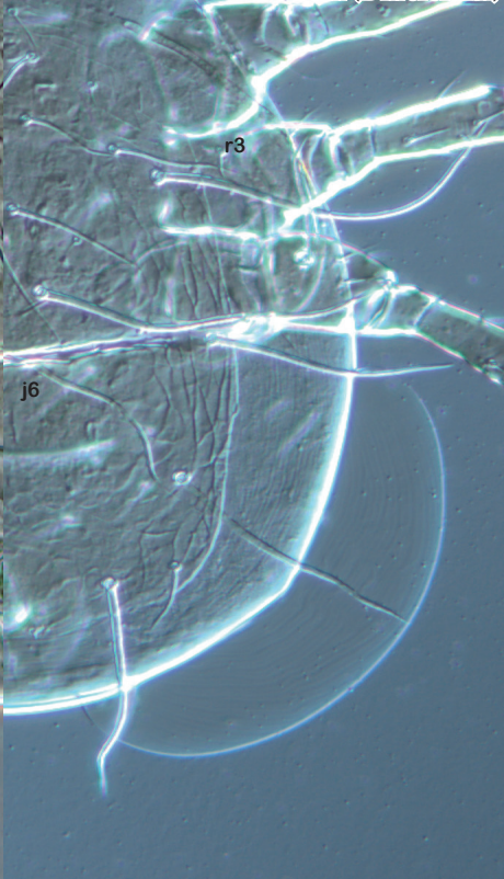
雄成虫鋏角 Chelicera (male)
